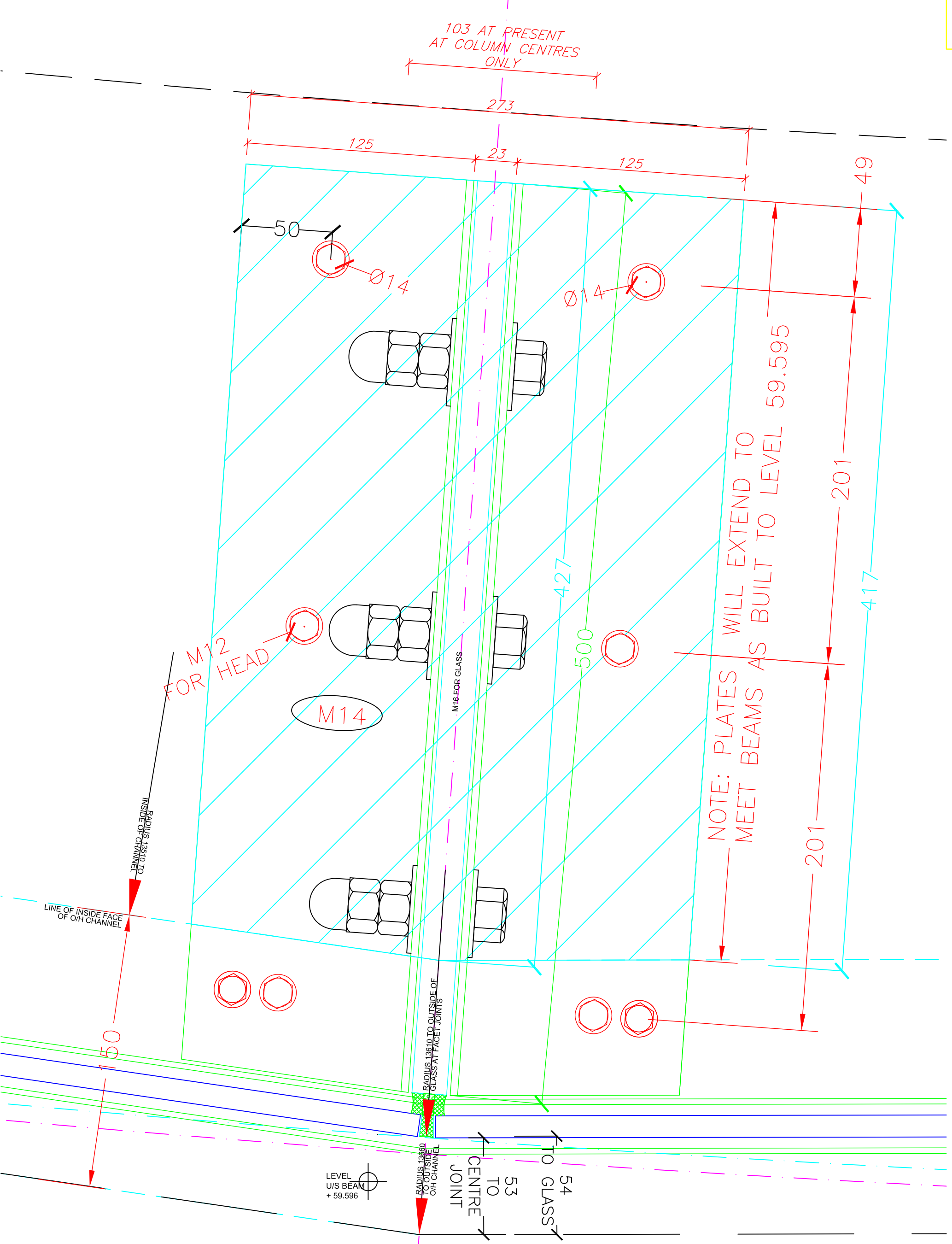
TYPICAL INVERTED HEAD BRACKET PLAN DETAIL AT BASE 1:2
